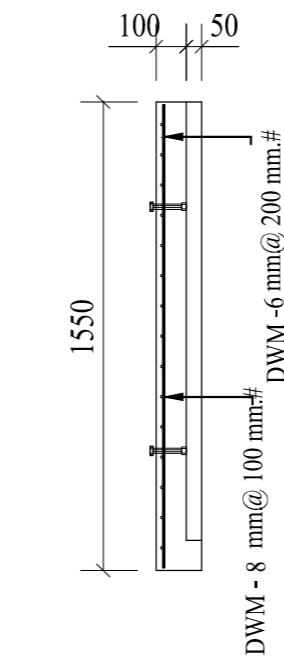
A - A (1:25)
