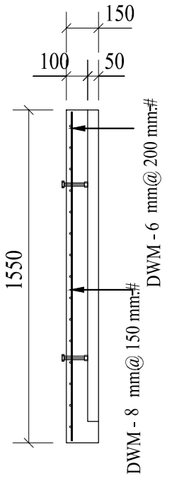
A - A (1:25)
