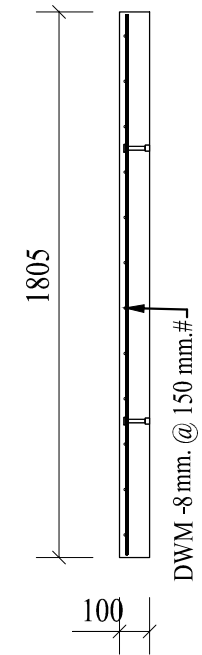
A - A (1:25)
