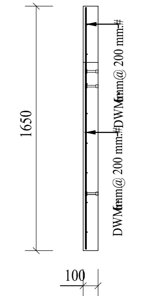
A - A (1:25)
