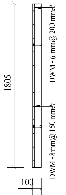
A - A (1:25)
