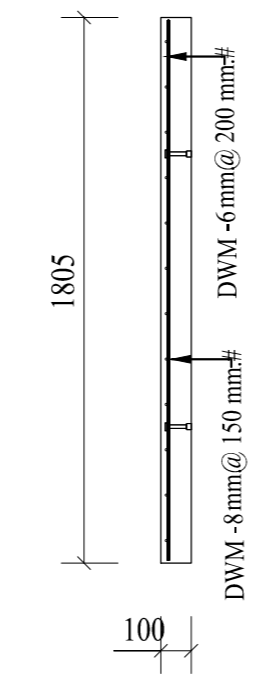
A - A (1:25)
