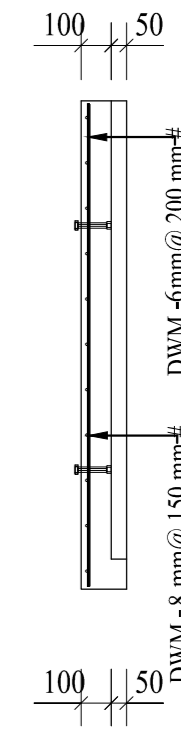
A - A (1:25)
